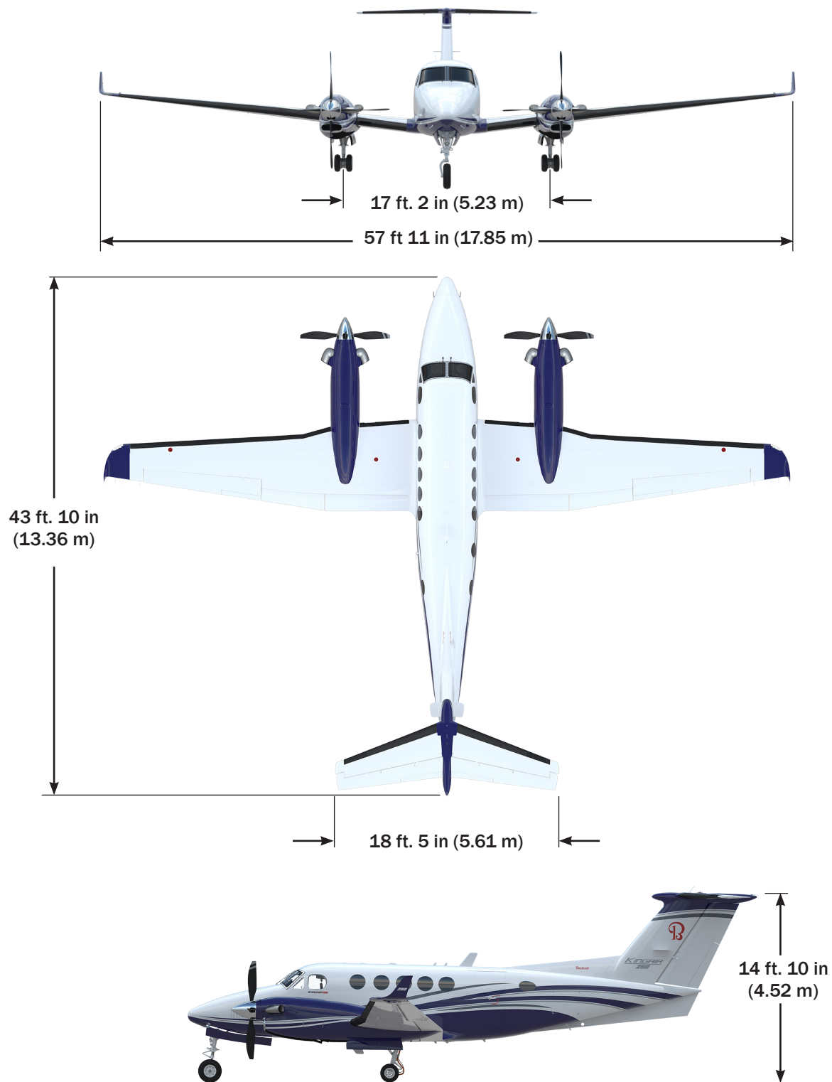
FIGURE 1 - KING AIR 250 EXTERIOR DIMENSIONS
