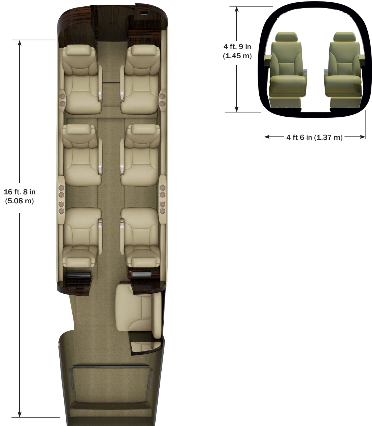
FIGURE 3 - KING AIR 250 STANDARD FLOORPLAN
